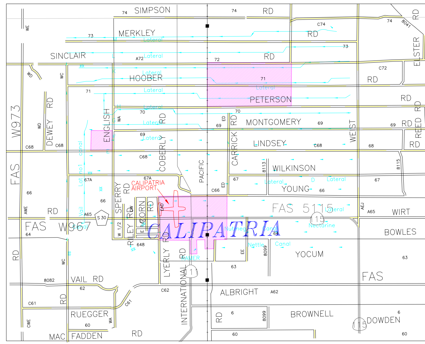
VICINITY MAP
